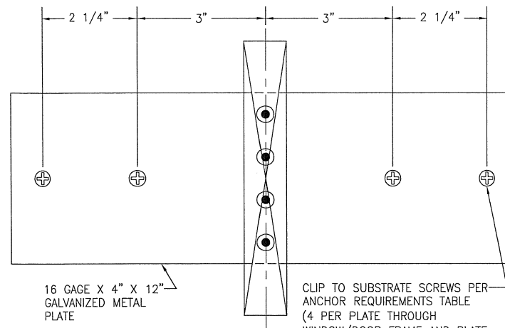
END CONNECTION OPTION 3B (SEE CONNECTION 3A FOR ATTACHMENT OF PLATE TO MULLION)
