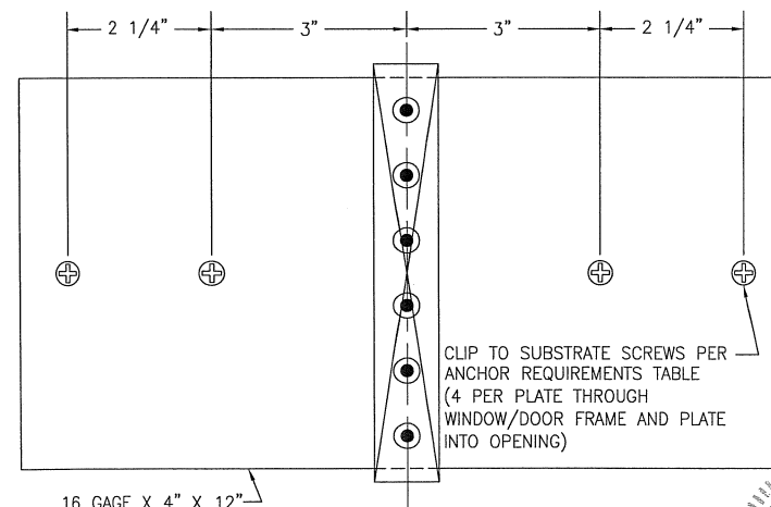
END CONNECTION OPTION 2B (SEE CONNECTION 2A FOR ATTACHMENT OF PLATE TO MULLION)
